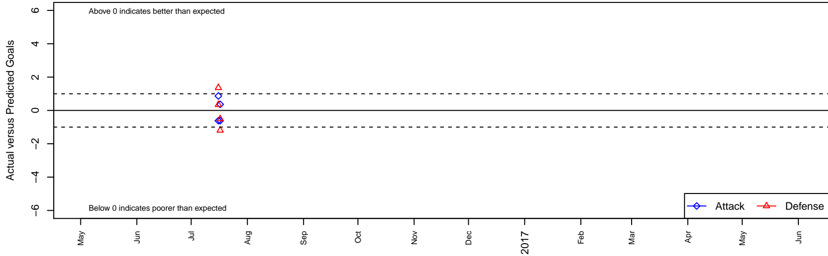
Albion SC Premier II B00 Dots are actual minus expected GF (blue circles) and GA (red triangles). Blue line is smoothed change in attack strength. Red is smoothed change in defense strength.
